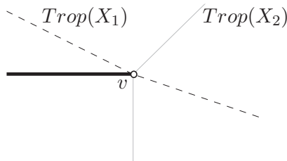
FIGURE 5. At least l-1 intersection points of X_1 and X_2 have valuation v .
