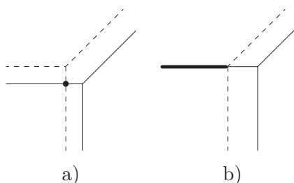
FIGURE 2. Transverse and non-transverse intersections. In both cases, \mu(E) = 1 .
