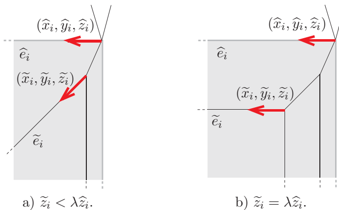
FIGURE 9. The slope of \widetilde{e}_i is bounded by the slope of \widehat{e}_i .
