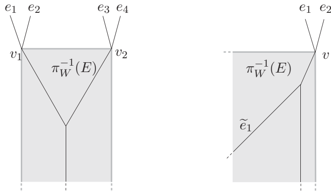
a) The compact case ( s = 0 ). b) The non compact case ( s > 0 ).
