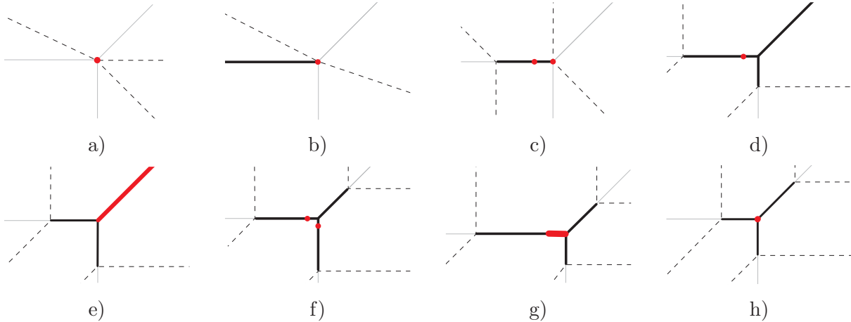
FIGURE 12. Description of \mathfrak{J}_L in all the possible cases.
